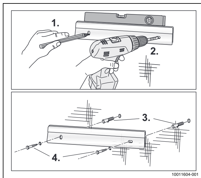
Man. 11 Installing the mounting rail on a concrete wall
