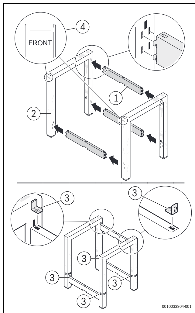
Man. 8 Installing the frame
