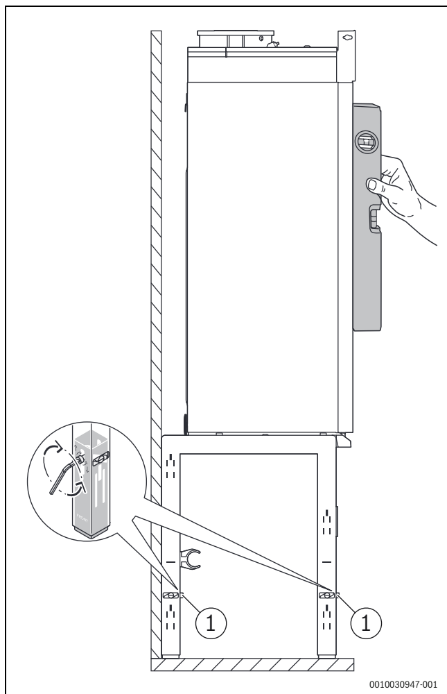
Man. 10 Align the boiler on the frame
