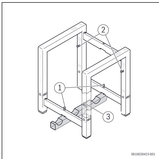
Man. 9 Secure the frame to the wall or floor
