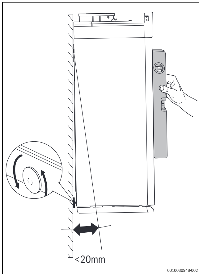
Мал. 12 Aligning the boiler on the wall
