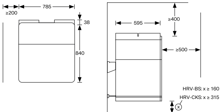
Logavent HRV176
