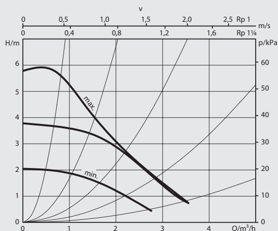
Logafix BUE-Plus-2 25/1-6 Logafix BUE-Plus-2 30/1-6
