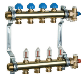
HKV-Top 5/4"
