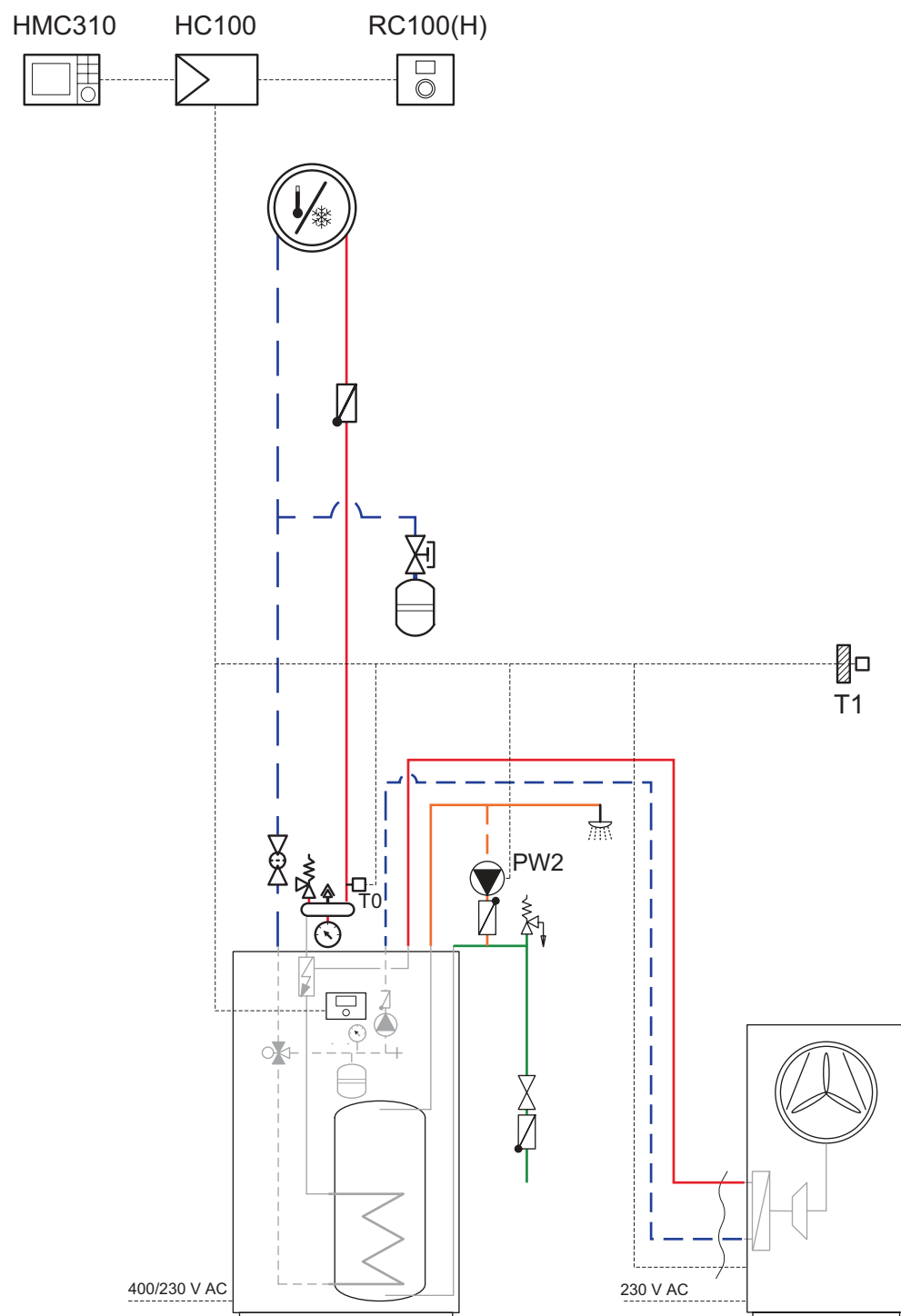
Logatherm WLW196i AR S+
